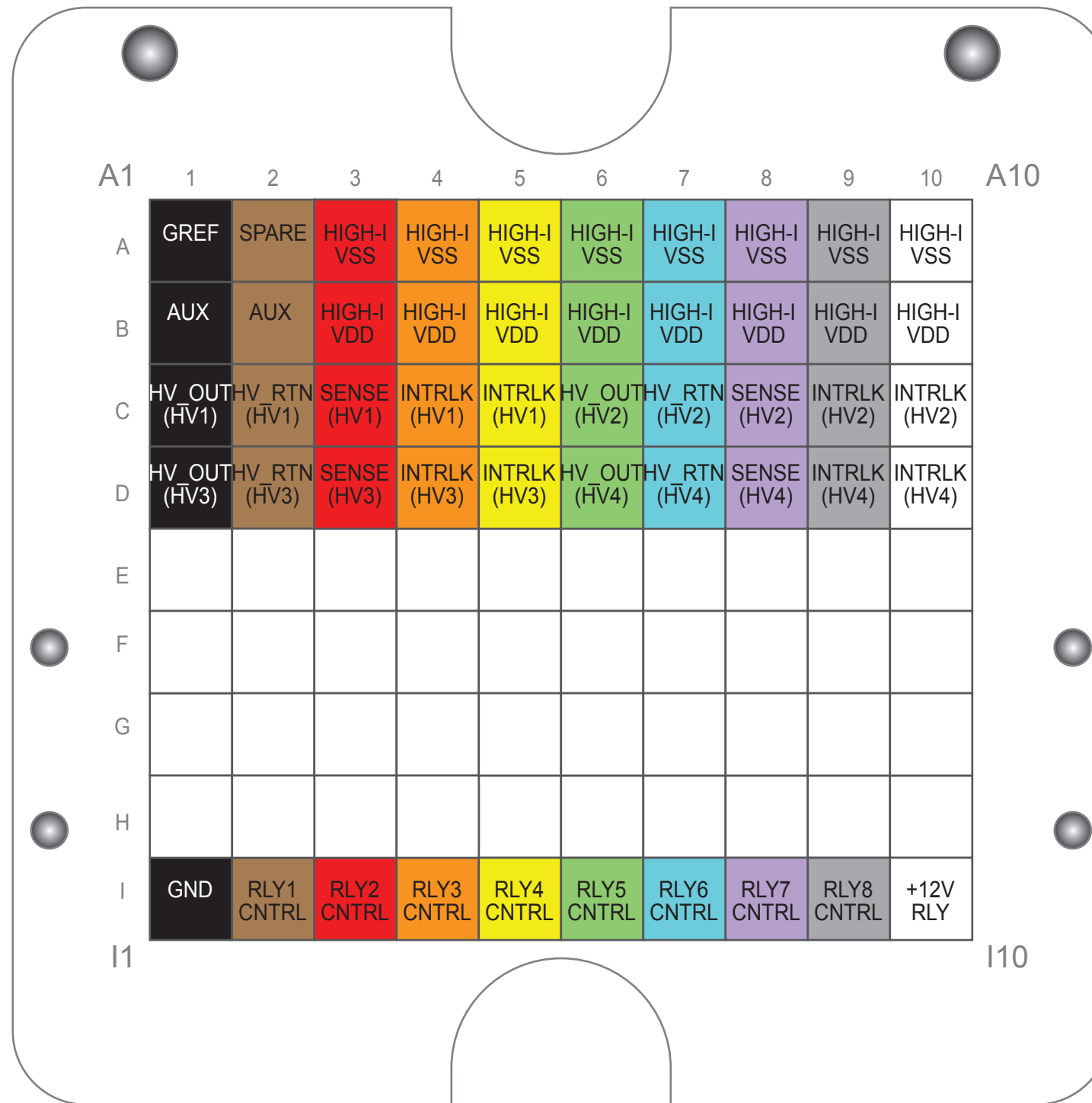
RI8589A Connections
