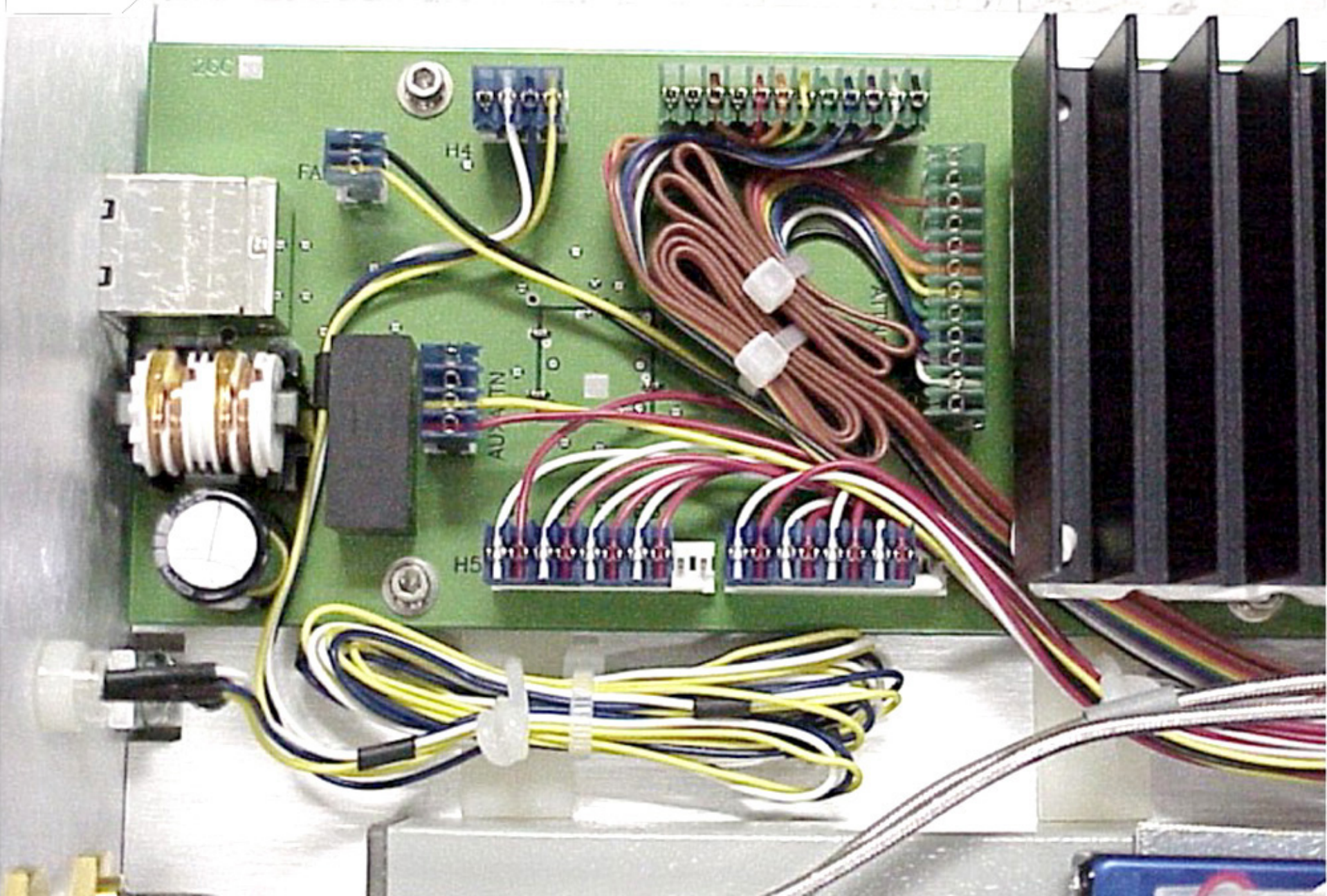
R17269A Source12 Output Module Closeup of PC Board Connections Image 2 of 8, 12/1/99
